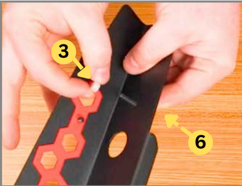
Step 2: Install Long 2.5mm Allen Bolt through the top of the Fender Shroud. Place Spacer on opposing side of Bolt.
