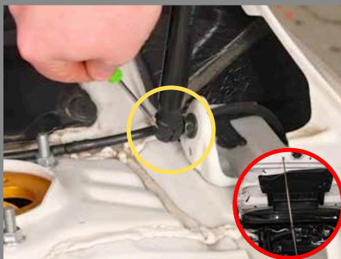
Step 5: Remove the Hood Strut from the bottom Ball Stud using a Screwdriver. NOTE: Support Hood using Prop Rod
